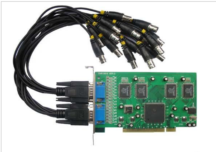
Multichannel capture card, Techwell 6801 10-bit ADCs Image Quality
